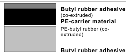
DENSOLEN®-N60 and DENSOLEN®-S20 design (different thicknesses)
